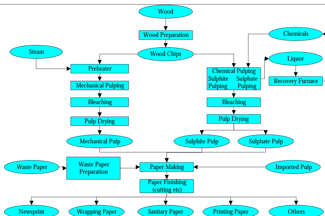
Figure 39 Schematic Diagram of Pulp and Paper Processes
