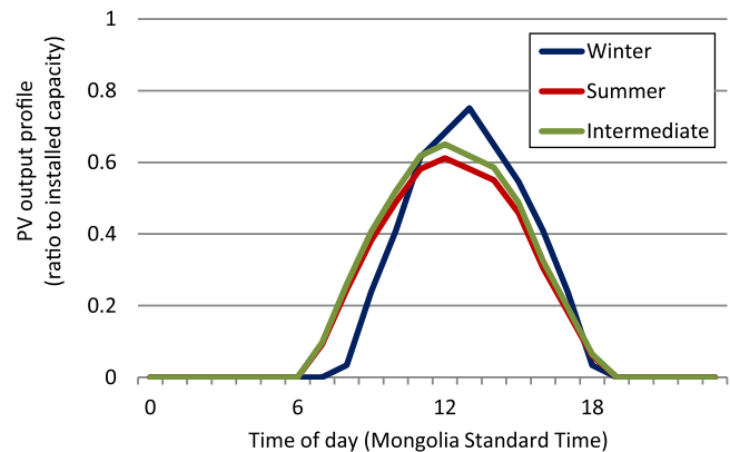
Fig. 7. Assumed daily output profile of PV in the Gobi Desert area (GD).
