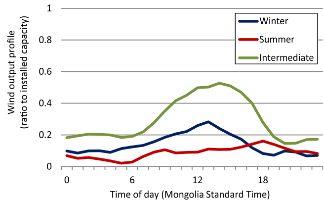
Fig. 6. Assumed daily output profile of wind in the Gobi Desert area (GD).
