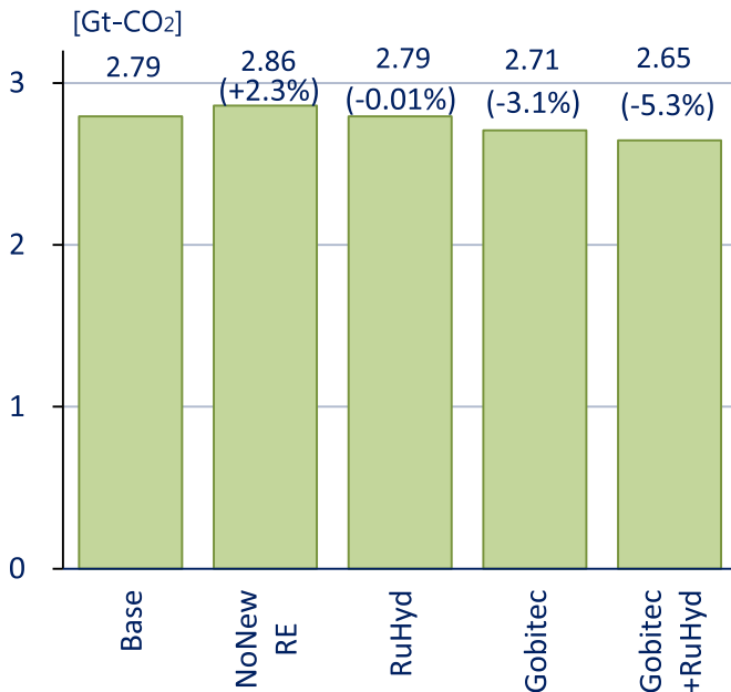
Fig. 11. CO 2 emissions in NEA region.
